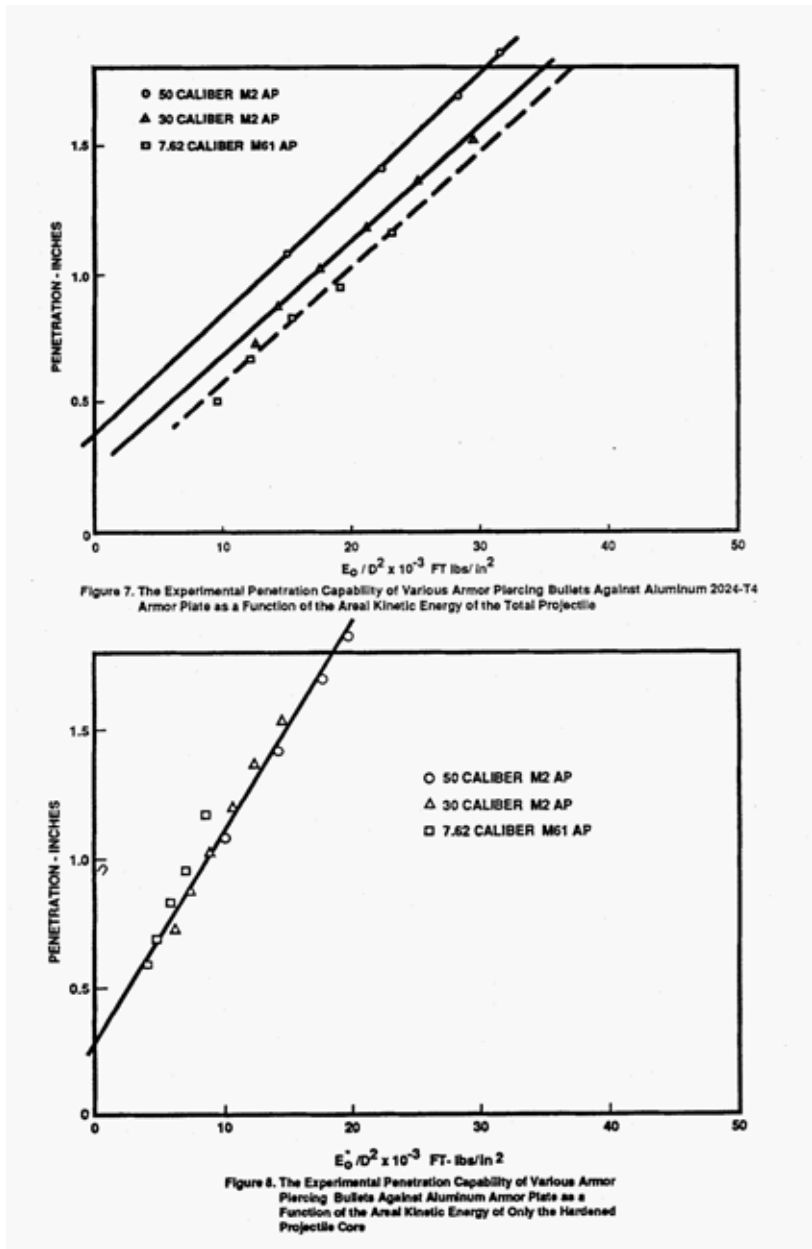
Figure 23. Penetration depth of ballistics rounds into aluminum plates as a function of projectile kinetic energy and projectile diameter [3].
