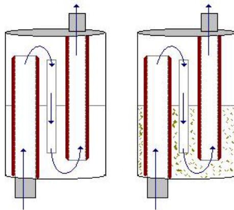
Figure 12. Muffler diagram, before and after packing
