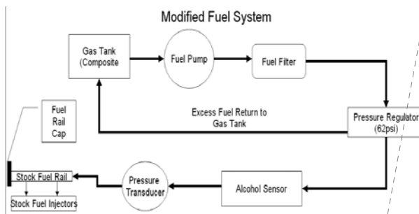
Figure 22. Modified Fuel System
