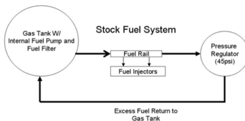
Figure 21. Stock Fuel System
