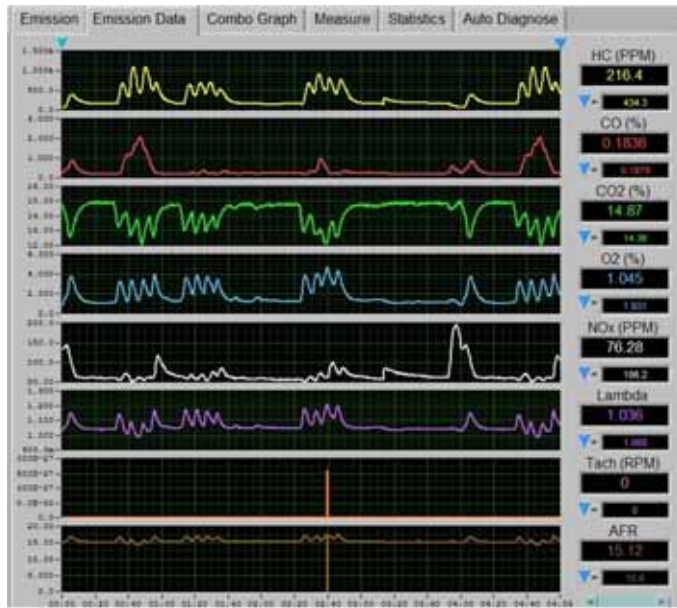
Figure 26. Emissions of UMaine Phazer running with MegaSquirt
